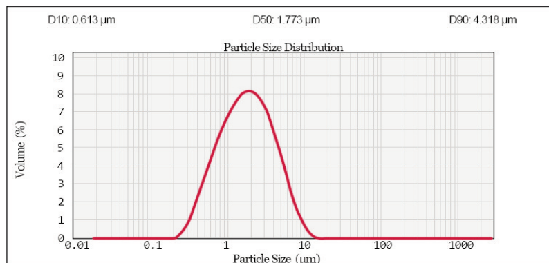
Ceroxid HD R1526 PSD laser particle size distribution analyzer
